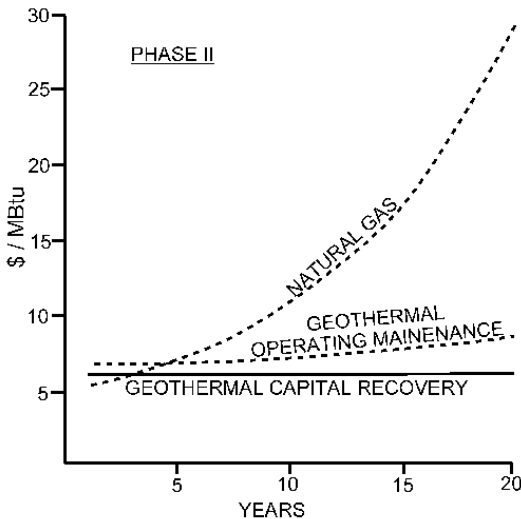
Figure 2. Phase II Unit Energy Cost Comparison (Lineau, 1981)
