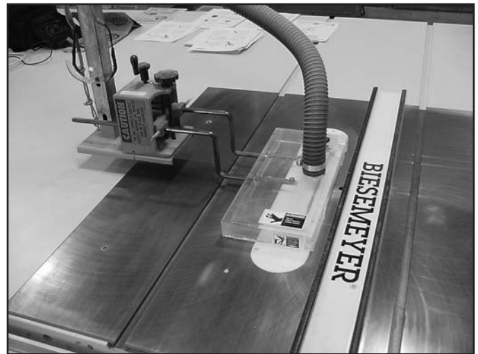
Coffee Creek Correctional Facility Manually adjustable "Brett-Guard."
