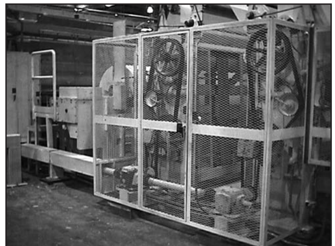
Fixed guard enclosing several belt drives.
