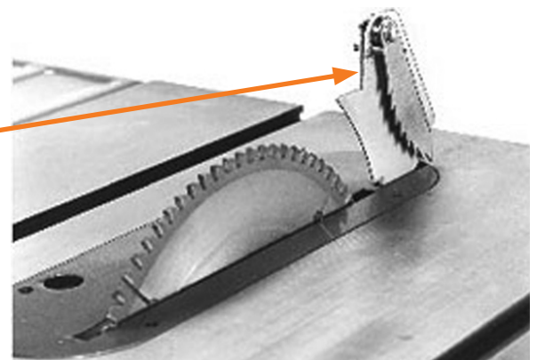
Biesemeyer Products/Delta Machinery Guard removed to show spreader device.
