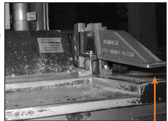
Missing “nose guard” on this jump saw.
