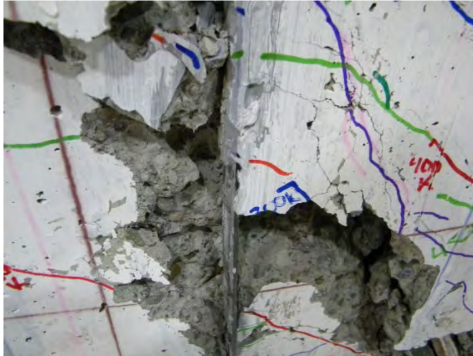
Figure 6.12: Example of debonding of NSM-CFRP
