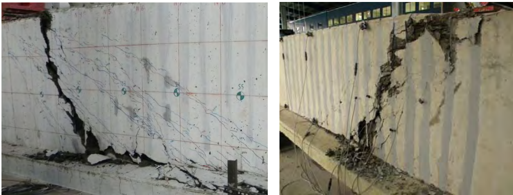
Figure 6.9: Specimen IT.7.18.6.M failure
