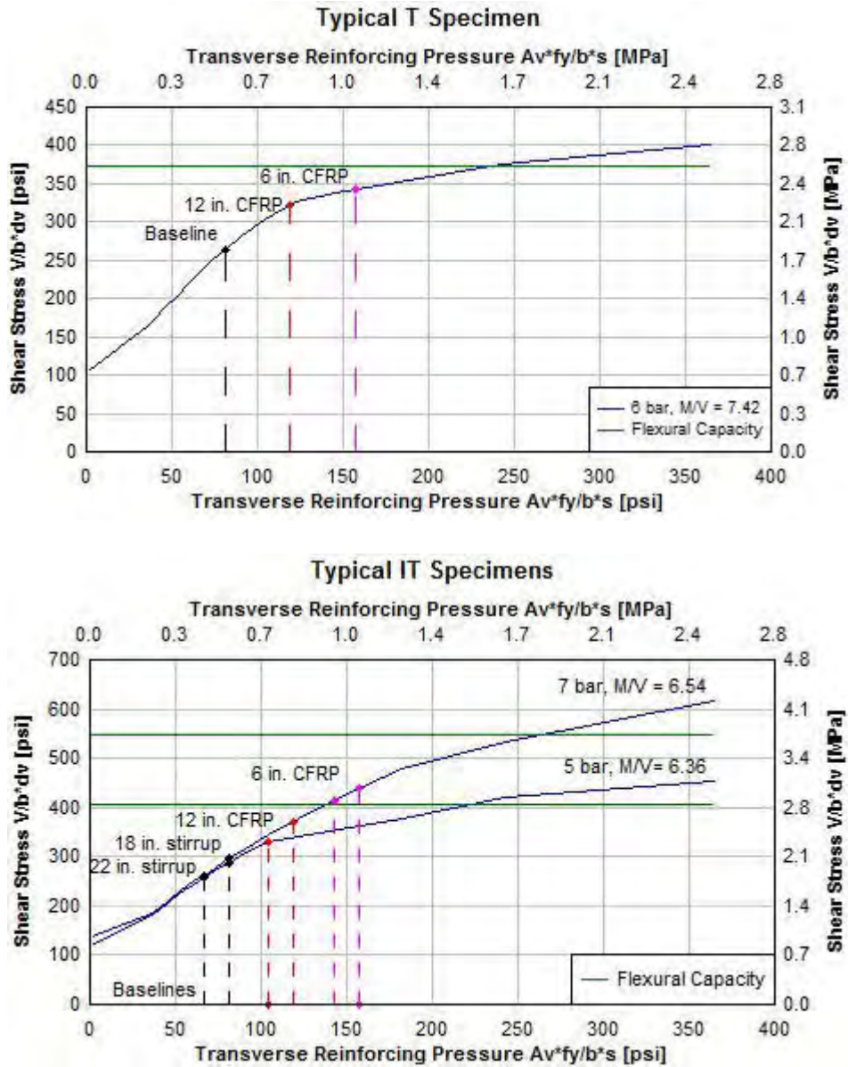
Figure 5.6: Shear stress vs. transverse reinforcing pressure interactions for specimen designs
