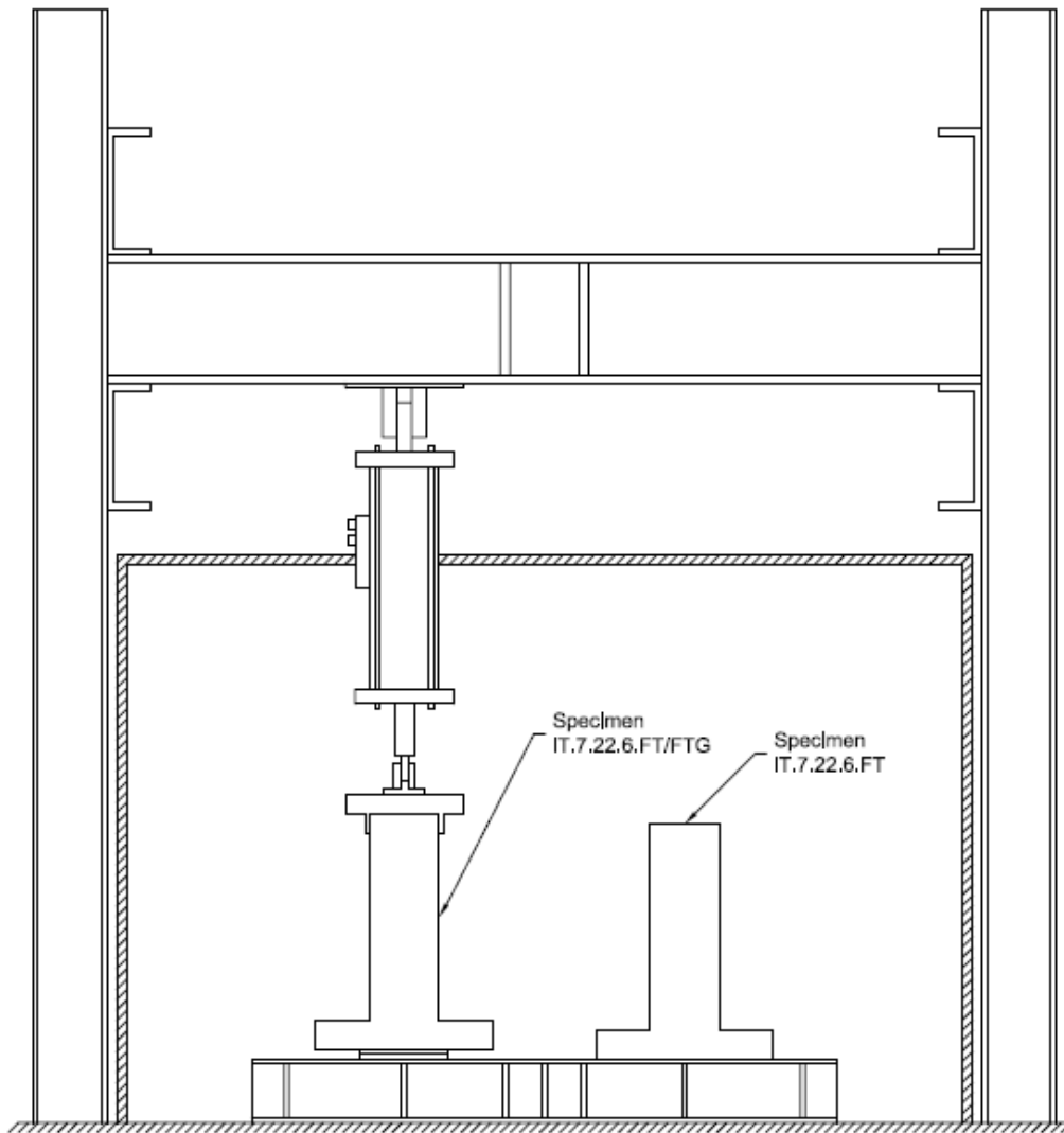
Figure 5.19: Freezer and fatigue setup
