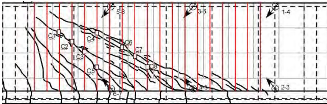
Figure 6.30: Specimen IT.7.22.6.S
